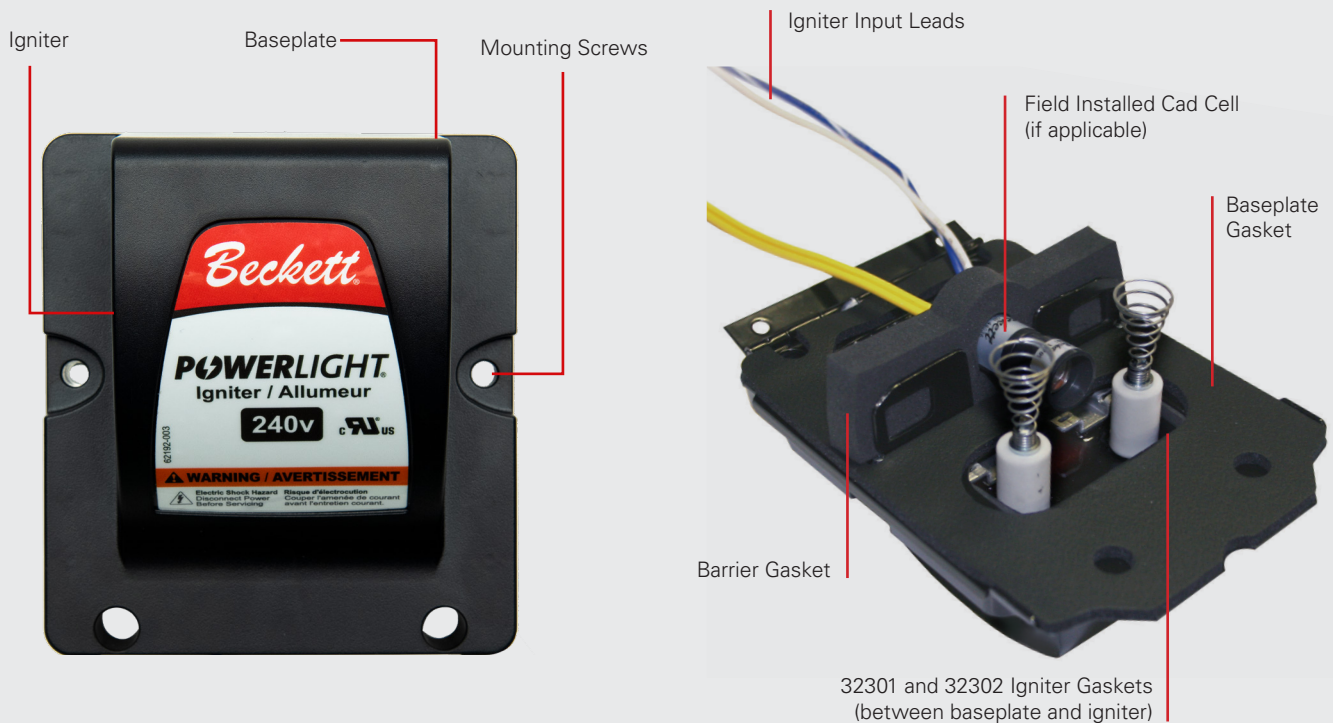
Figure 1 — Igniter Assembly Components (5250001U shown. Other models will have different baseplates and terminals.)
